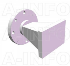
LB-22-15-ASPO Standard Gain Horn Antenna 33-50GHz 15dB Gain Rectangular Waveguide Interface
